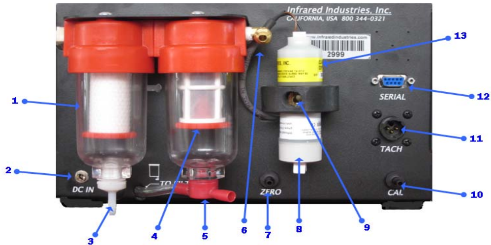
Figure 2: Rear Panel
