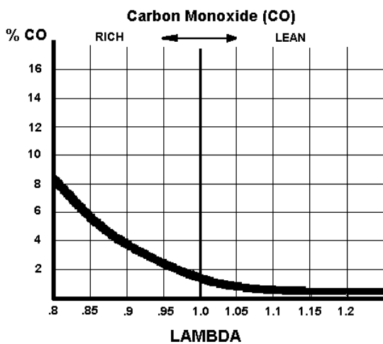
Figure 7 CO Vs Lambda
