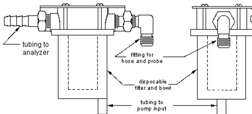
Figure 3: Filter Assemblies
