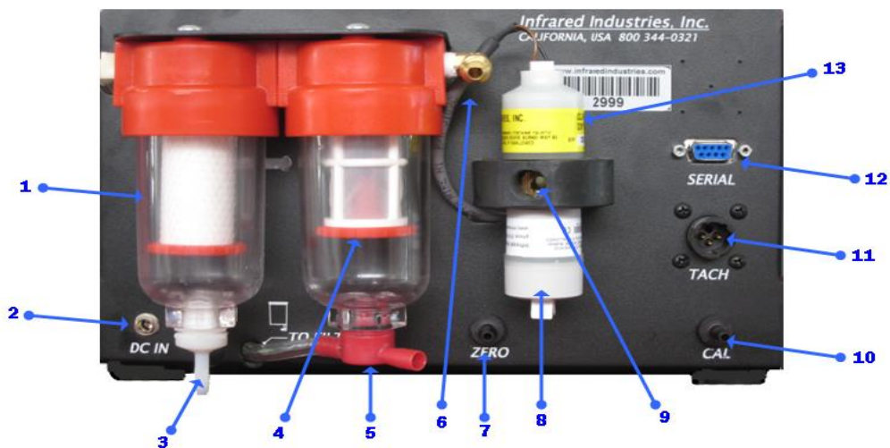
Figure 2: Rear Panel
