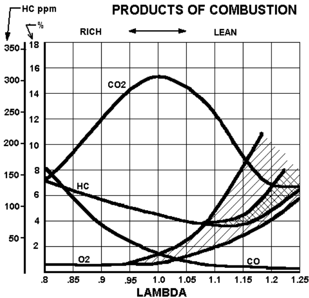
Figure 10 Combustion Products Vs Lambda
