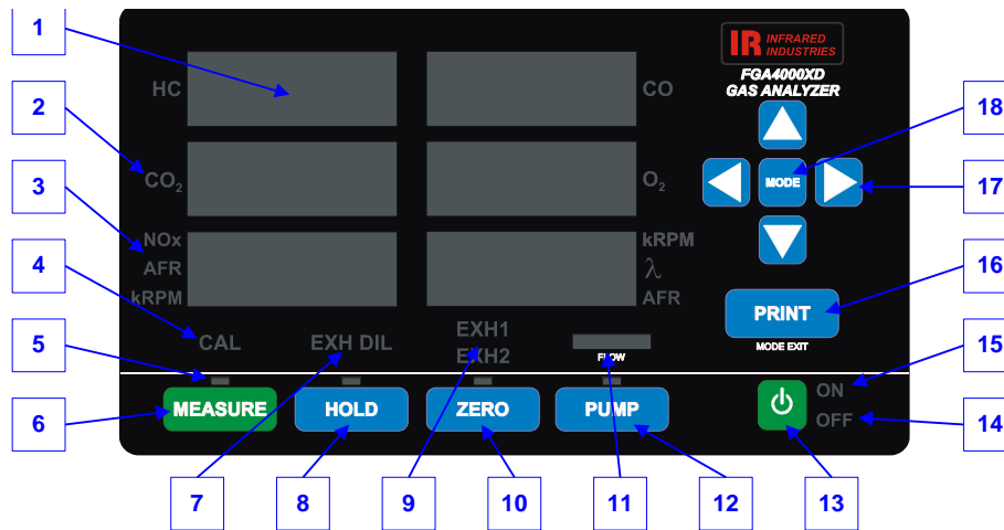
Figure 1: Front Panel
